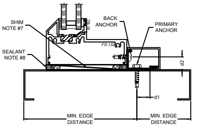
SILL
